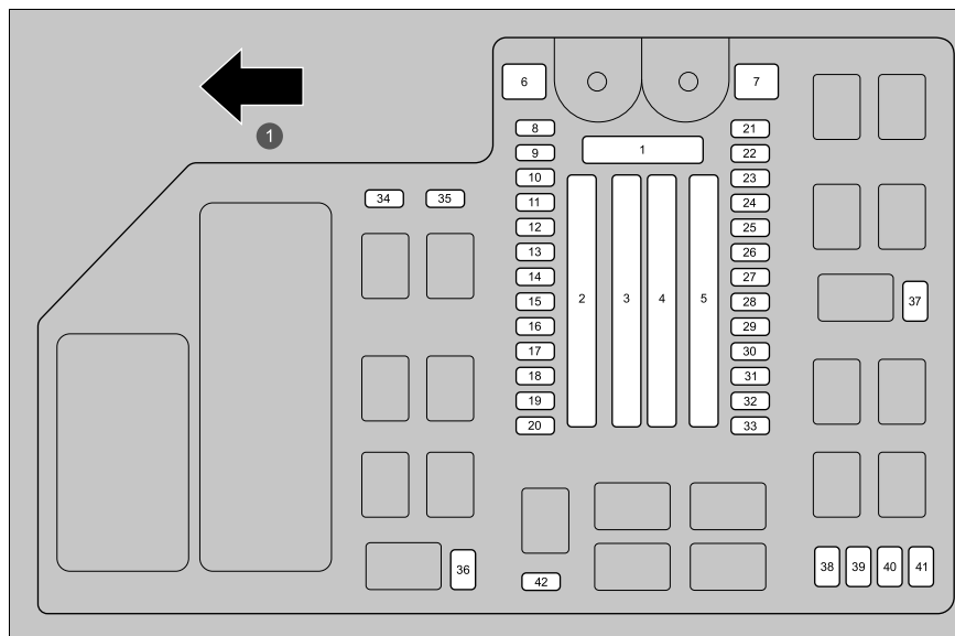
1 Front
